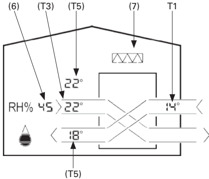
Heat recovery active
